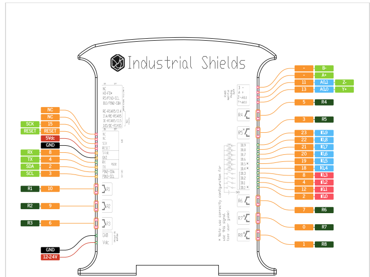
Ardbox Relay DALI Communication Zone Pinout
