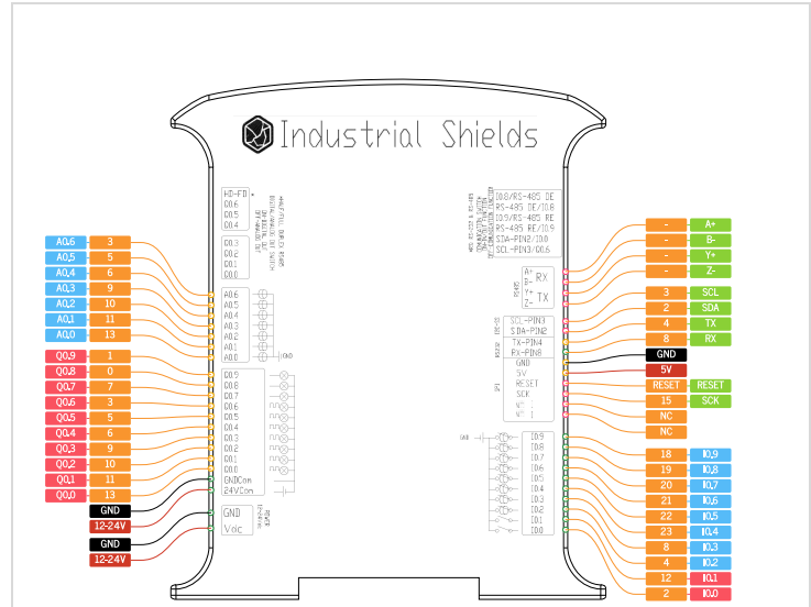
Ardbox Analog DALI Communication Zone Pinout
