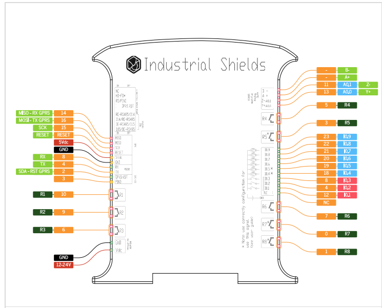
Ardbox Relay GPRS Communication Zone Pinout
