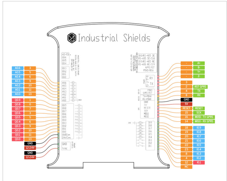
Ardbox Analog GPRS Communication Zone Pinout
