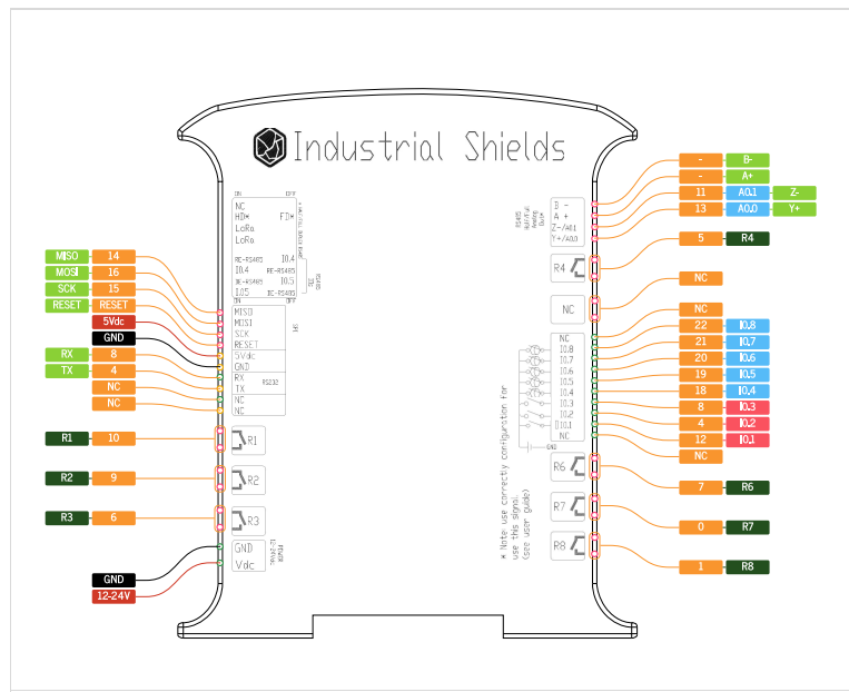
Ardbox Relay LoRa Communication Zone Pinout
