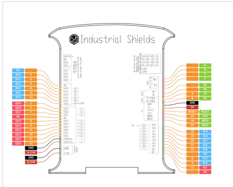
Ardbox Analog LoRa Communication Zone Pinout
