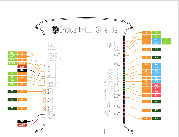
Ardbox Relay WIFI/BLE Communication Zone Pinout
