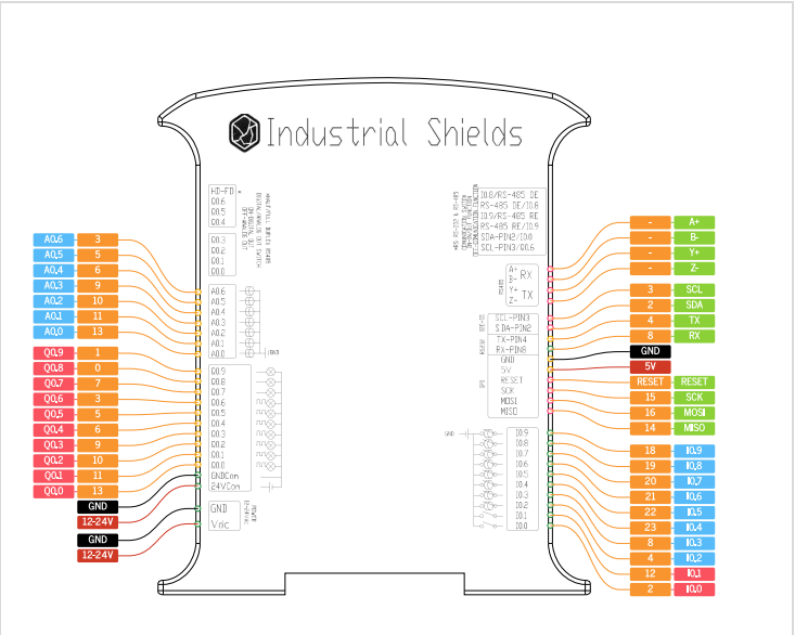
Ardbox Analog WIFI/BLE Communication Zone Pinout
